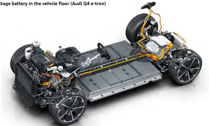
High-voltage battery in the vehicle floor (Audi Q4 e-tron)
