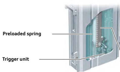
Latching mechanism
