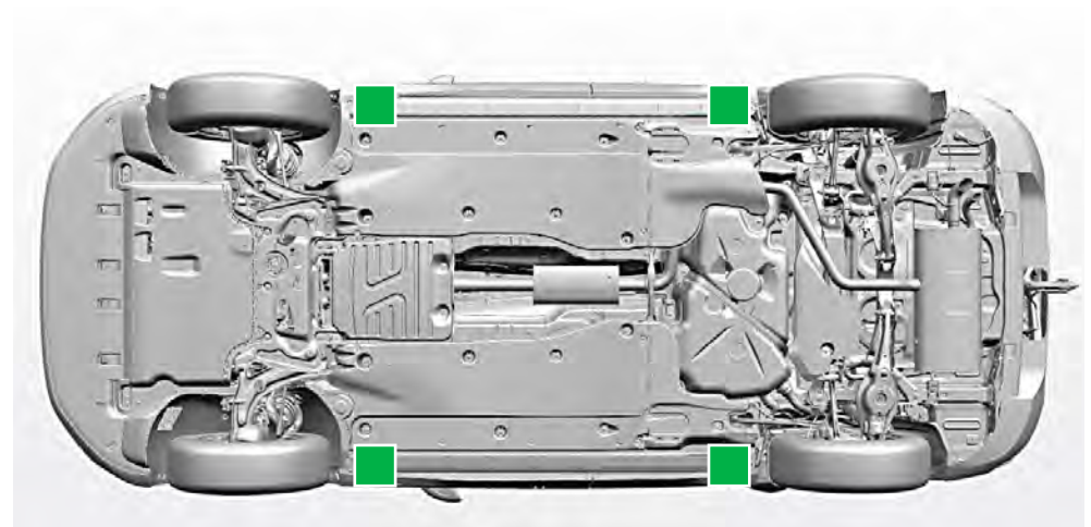
Suitable lifting points using the Audi A5 as an example
